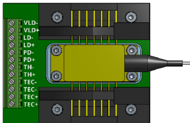
BTF100 terminal block connections
