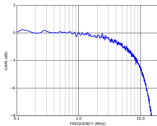
PDX10B-80-DC-SI (80 kV/A) frequency response
