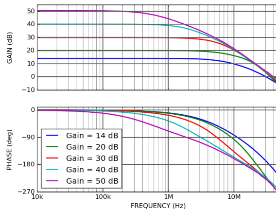
AMP200-1M (1 M \Omega ) frequency response
