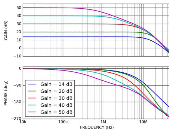
AMP200-10k (10 k \Omega ) frequency response
